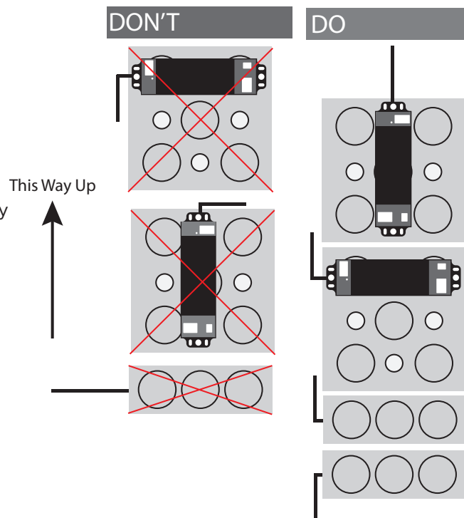
FIGURE 1 - ANTENNA ORIENTATION
