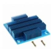
ATS-18H-105-C3-R1 HEATSINK 45X40X9.5MM XCUT T412 Advanced Thermal Solutions Inc.
