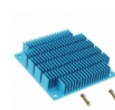
ATS-03F-207-C3-R0 HEATSINK 60X60X12MM XCUT T412 Advanced Thermal Solutions Inc.
